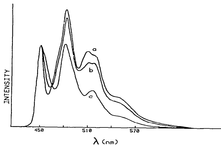
Fig. 1. Emission spectra of (a) [\text{Rh}(\text{bpy})_3]^{3+} , (b) [\text{Rh}(\text{bpy})_2(\text{phen})]^{3+} and (c) [\text{Rh}(\text{phen})_3]^{3+} in ethanol at 77 K.
