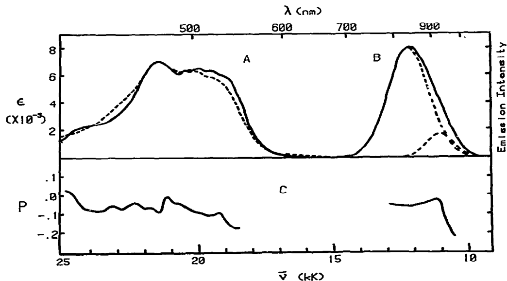
Fig. 6. 77 K corrected excitation (A, —); absorption (A, - - - -); emission (B, —) and excitation and emission polarization spectra (C) for \text{Ir}(\text{SacSac})_3 . The deconvolution of the emission into two Gaussian curves is shown.
